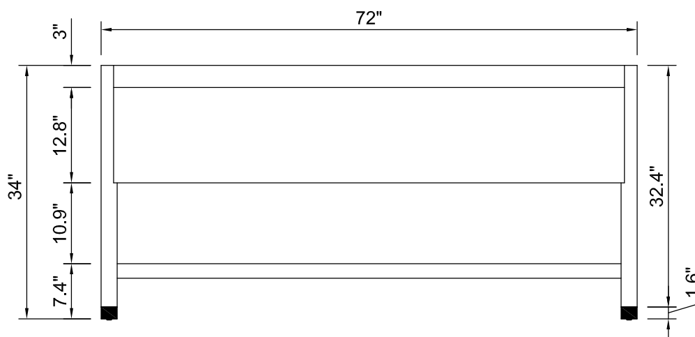
BACK VIEW
