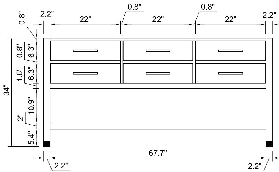
FRONT VIEW
